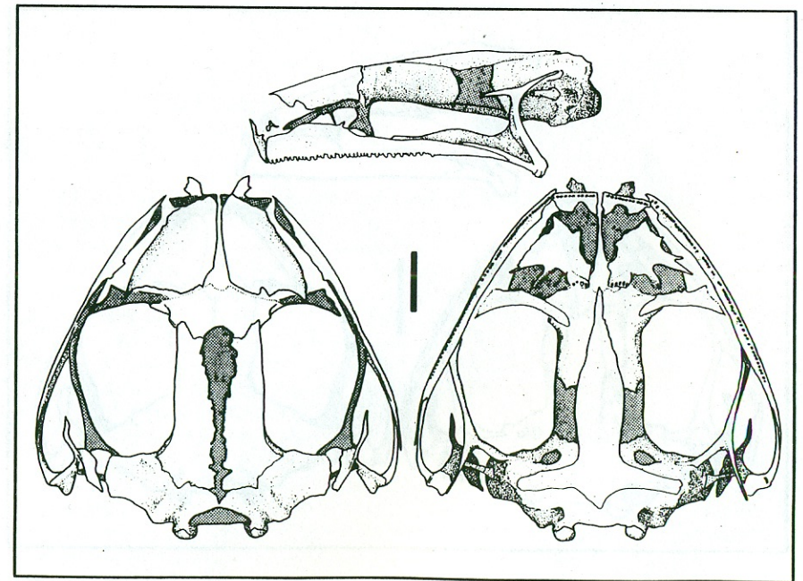
Fig. 9. Cranium of Eleutherodactylus discoidalis , KU 206433. Scale equals 2 mm.
