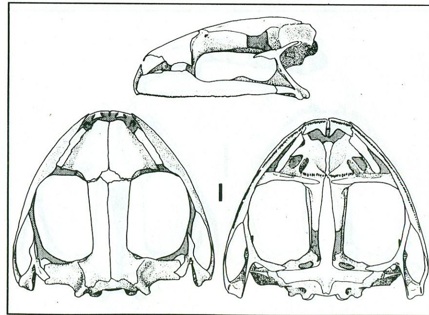
Fig. 8. Cranium of Eleutherodactylus dolops , KU 165866. Scale equals 2 mm.
